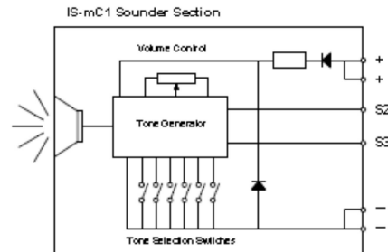
Fig 1 Simplified block diagram
