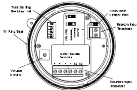
Fig 2 Location of field terminals and controls.
