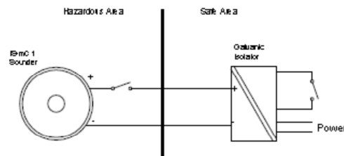
Fig 9 Sounder single stage alarm using galvanic isolator.
