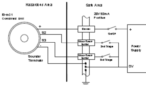
Fig 6 Sounder multi stage alarm using Zener barriers.
